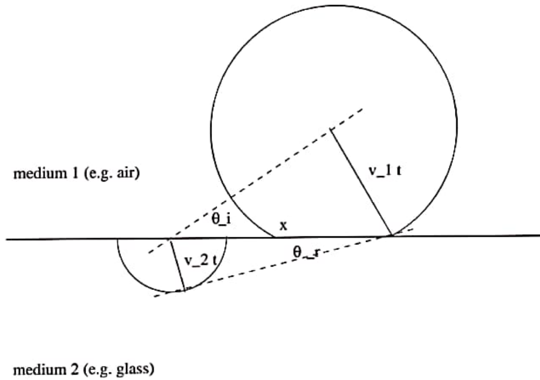
Figure 2.1: Refraction
