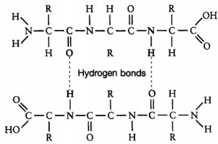
The Hydrogen Bonding between Proteins
