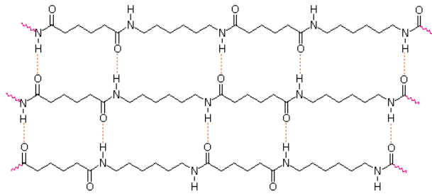
The Hydrogen Bonding between Nylon Polyamides
